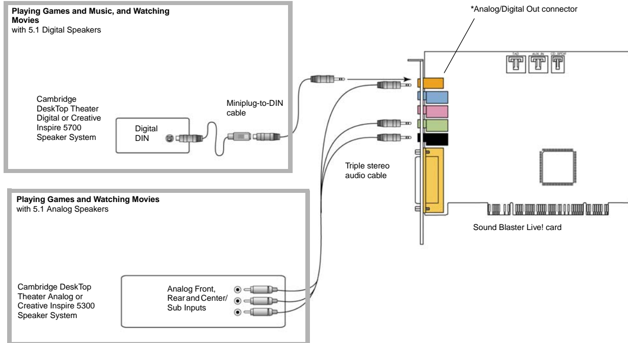
Figure 1-6: Connecting speakers to the Sound Blaster Live! card.
