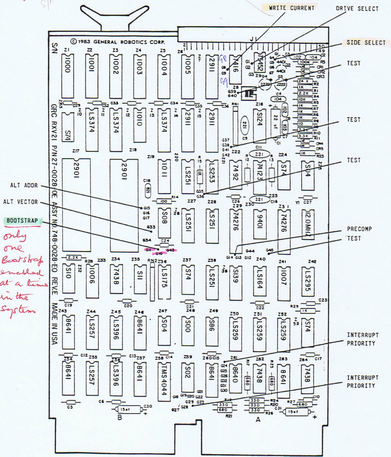
Figure 2-1: Configuration Jumper locations REV. E
