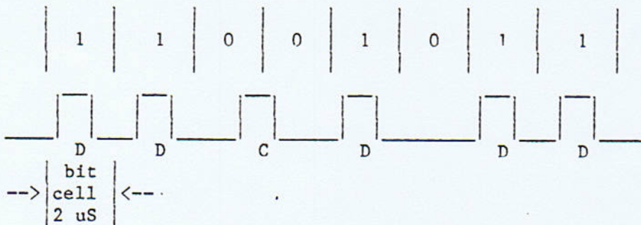
Figure 1.3 MFM Recording Characteristics
