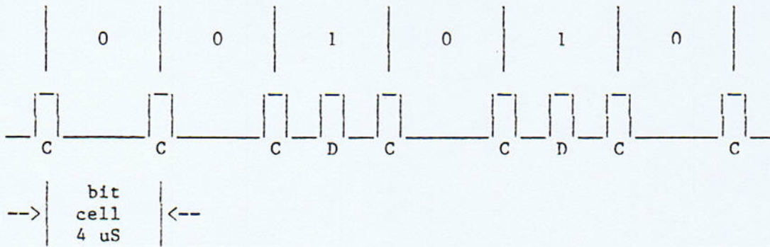
Figure 1.2 FM Recording Characteristics
