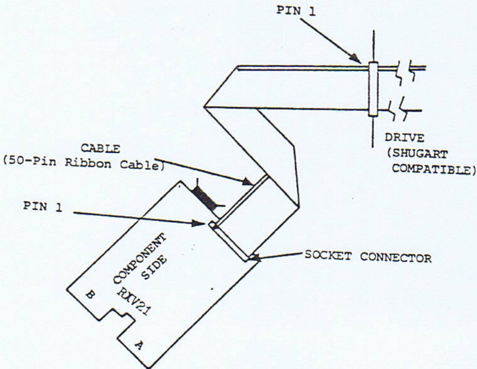
Figure 2.2 Drive/Controller Cabling
