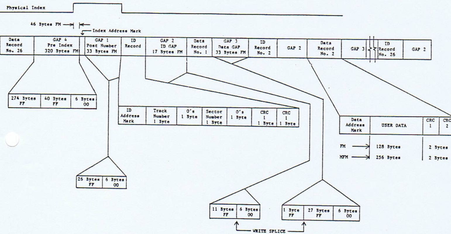
Figure 1.1 Logical Track Format
