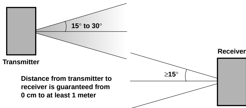
Figure 2. IrDA Viewing Angle and Distance.
