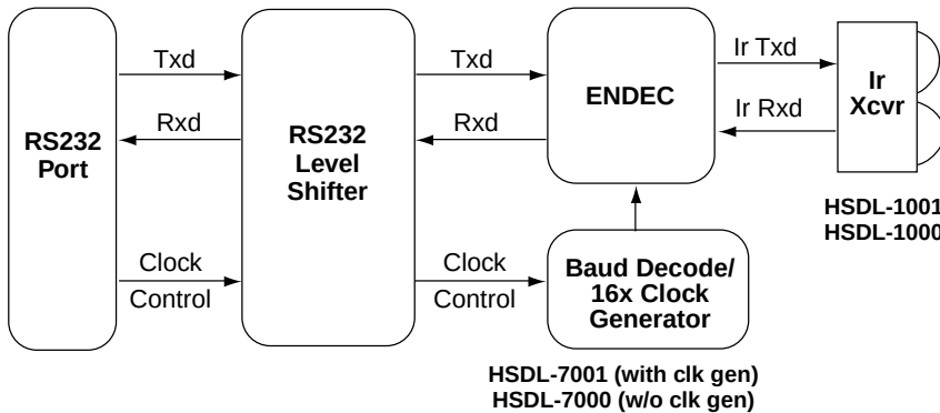
Figure 15. RS232 Adapter.
