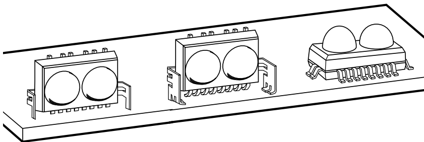
Figure 20b. HSDL-1100 Lead Bend Options.
