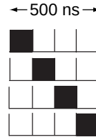
Figure 5. 4 PPM Modulation.
