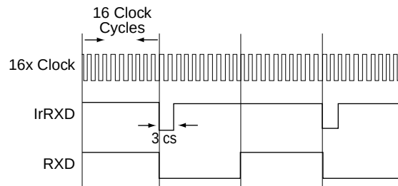
Figure 13. Ir Receive.
