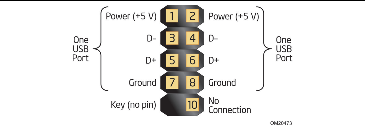
Figure 15. Connection Diagram for Front Panel USB 2.0 Headers
