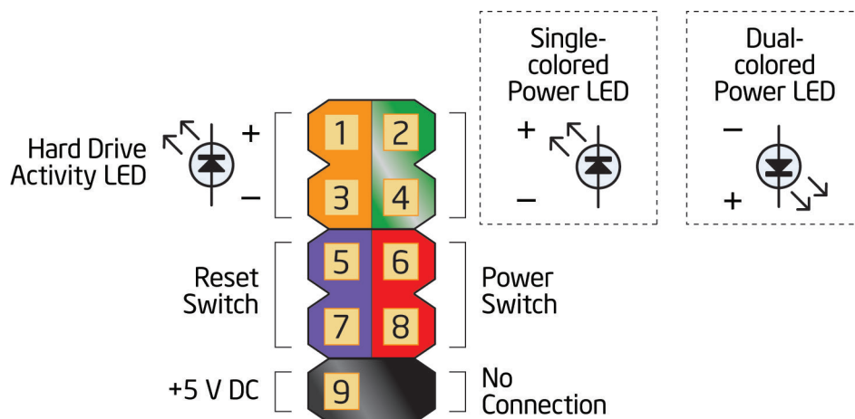
Figure 14. Connection Diagram for Front Panel Header
