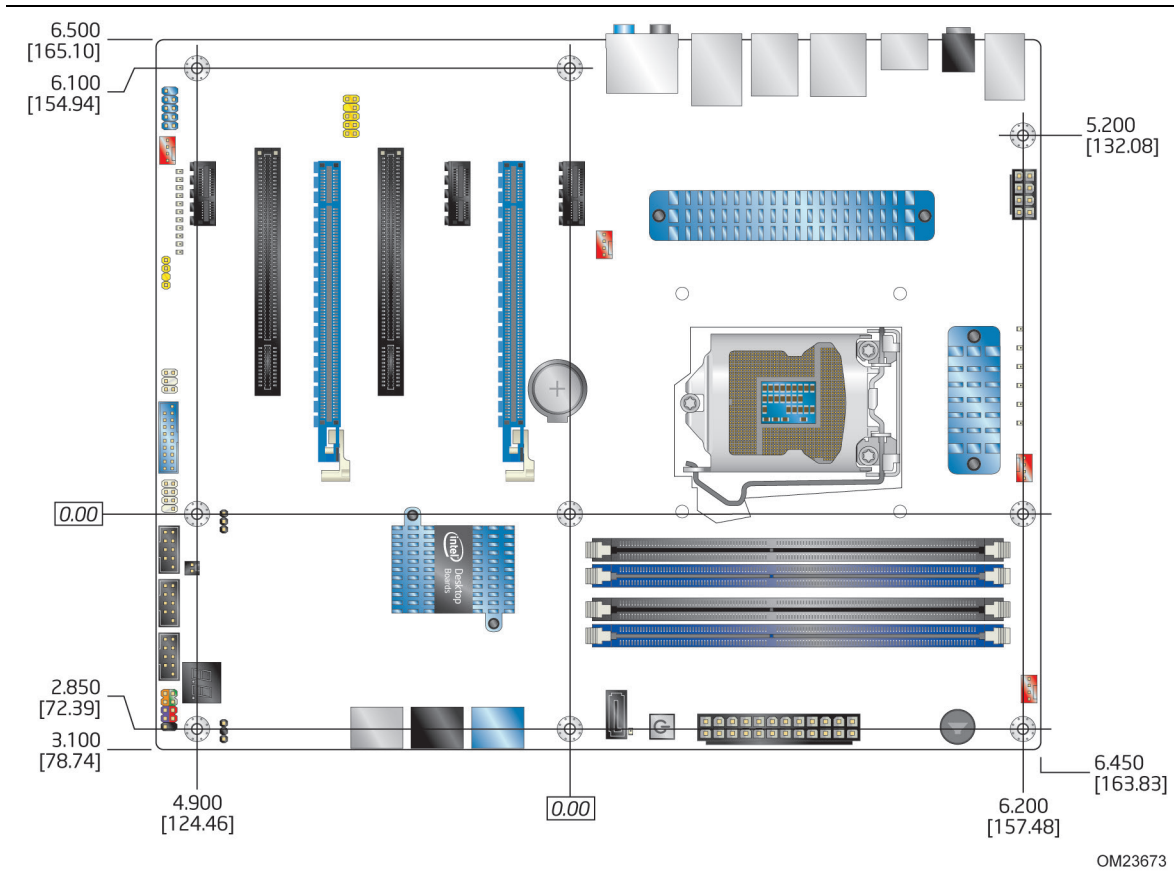
Figure 17. Board Dimensions
