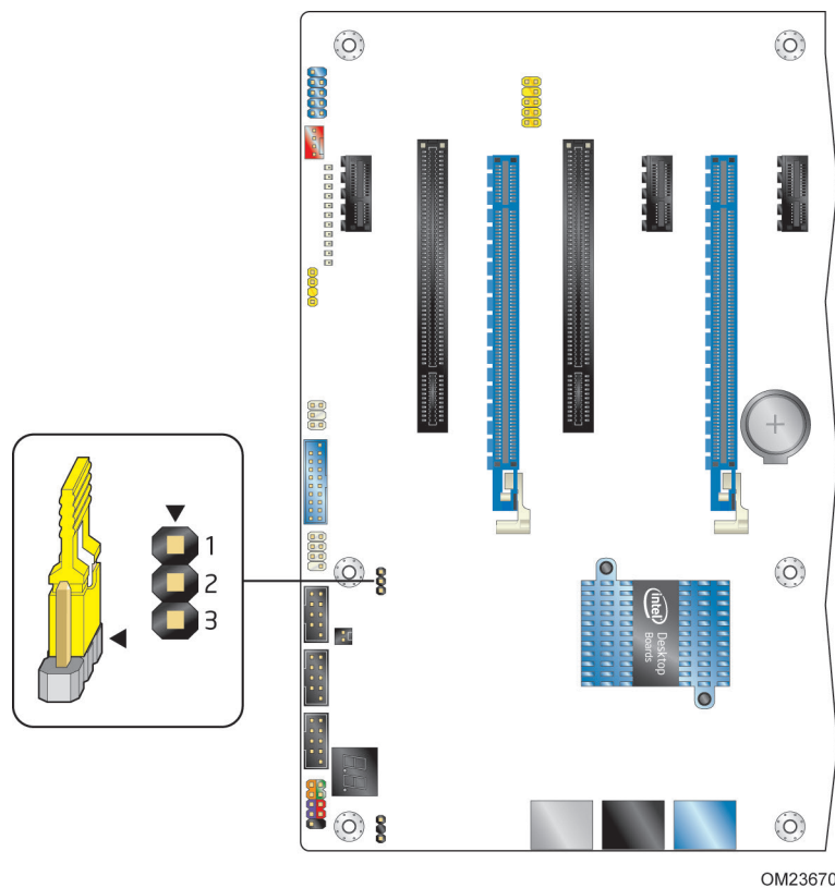
Figure 16. Location of the Jumper Block
