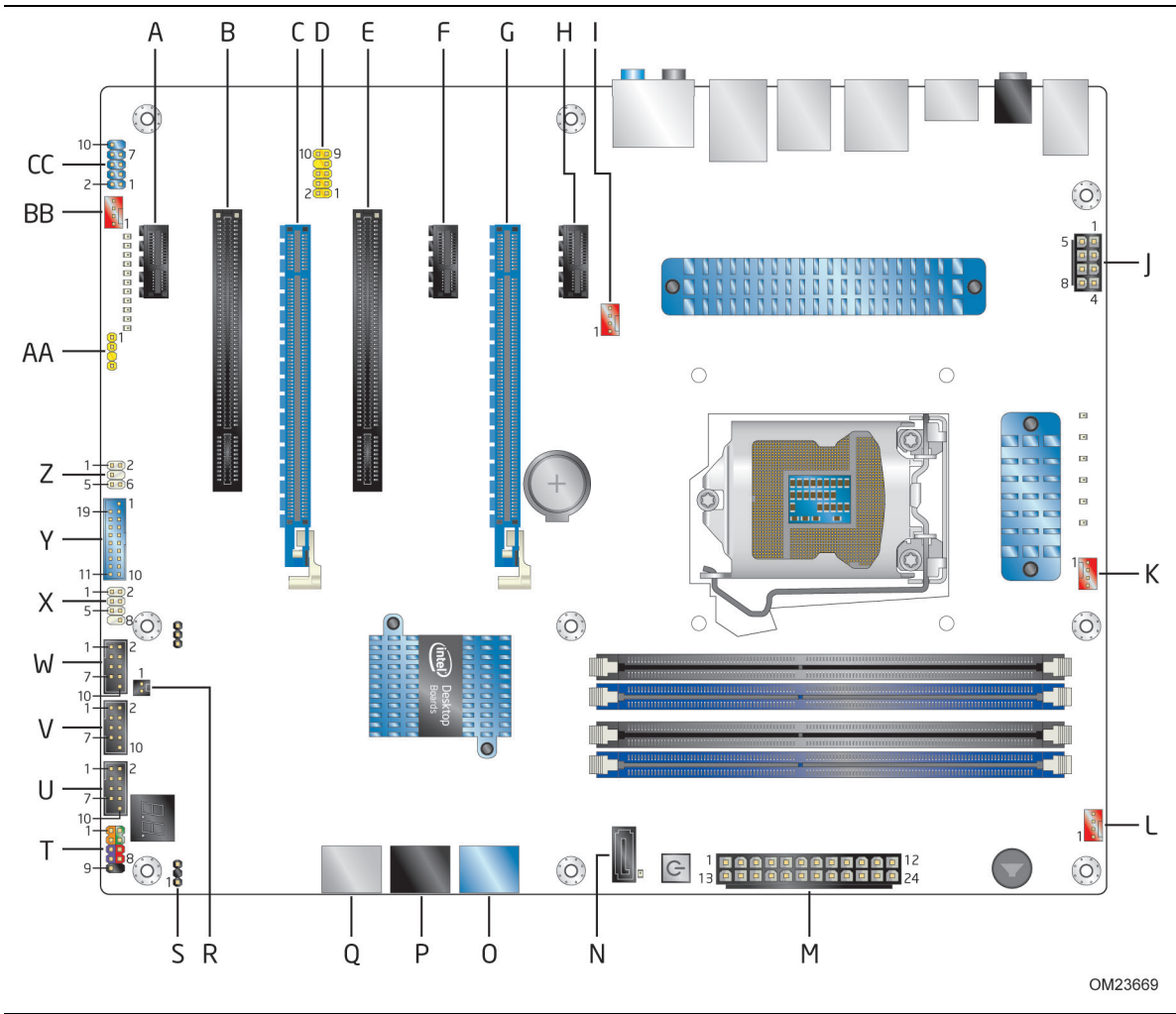
Figure 13. Component-side Connectors and Headers
