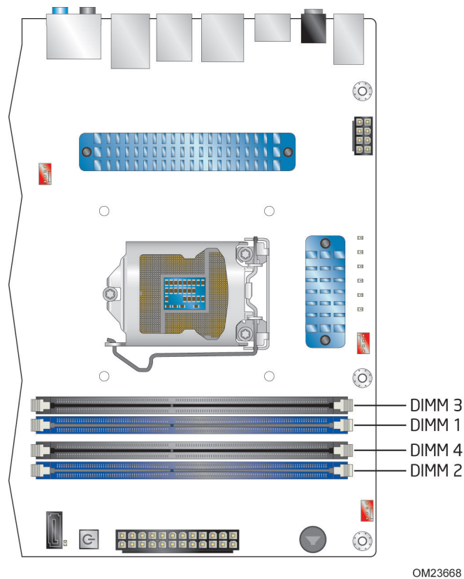
Figure 3. DIMM Configuration
