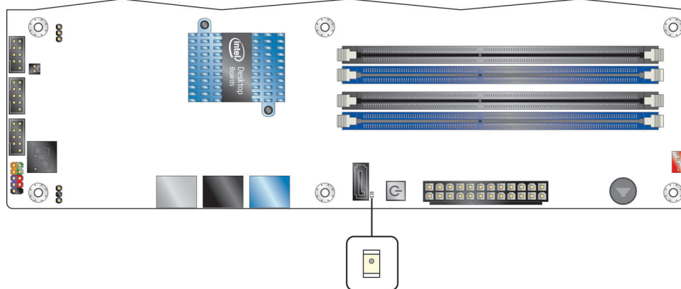
Figure 7. Location of the Standby Power LED
