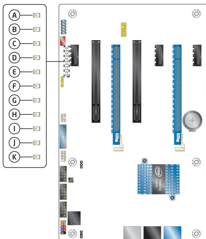
Figure 9. Location of Board Status LEDs
