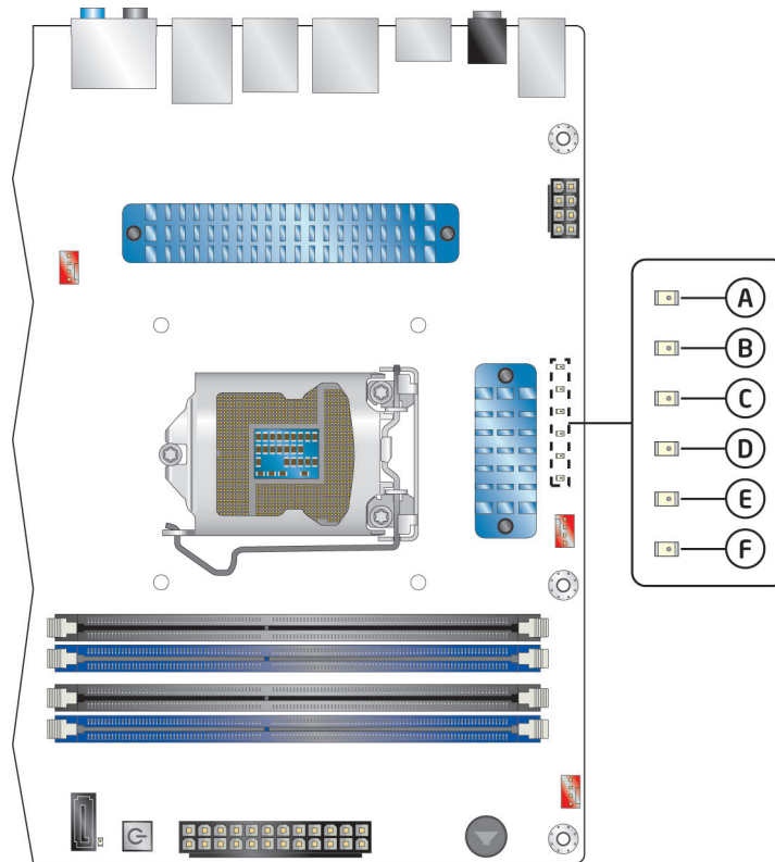
Figure 8. Location of the VR Status LEDs
