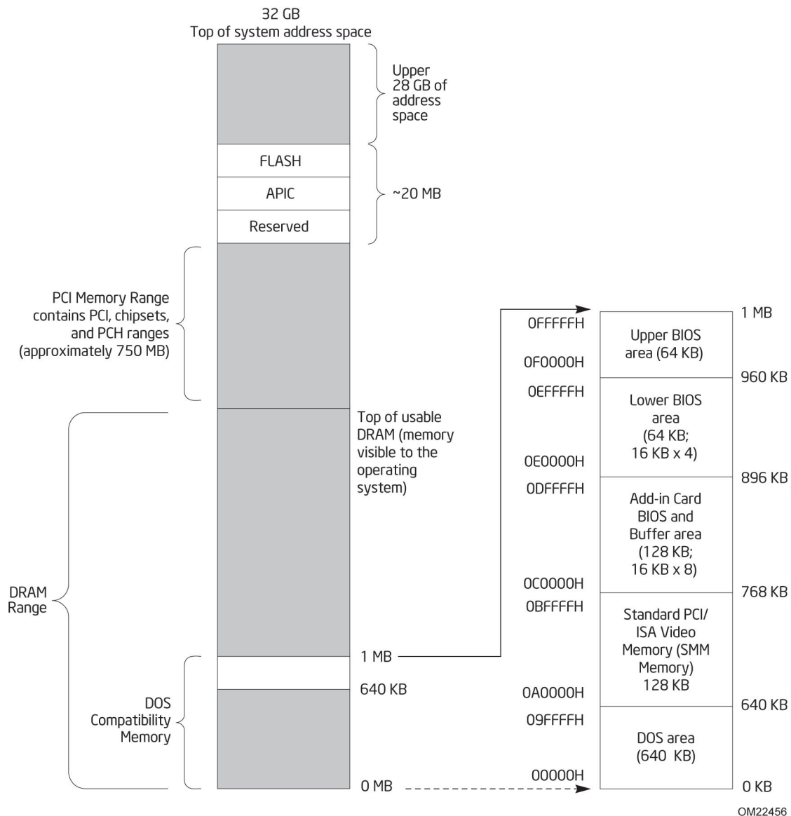
Figure 11. Detailed System Memory Address Map
