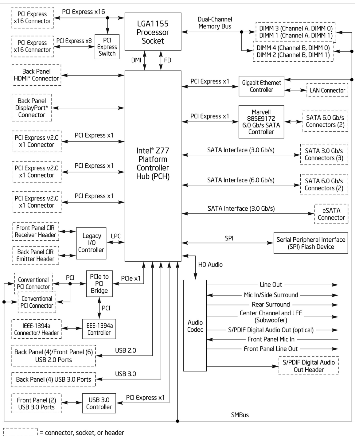
Figure 2. Block Diagram
