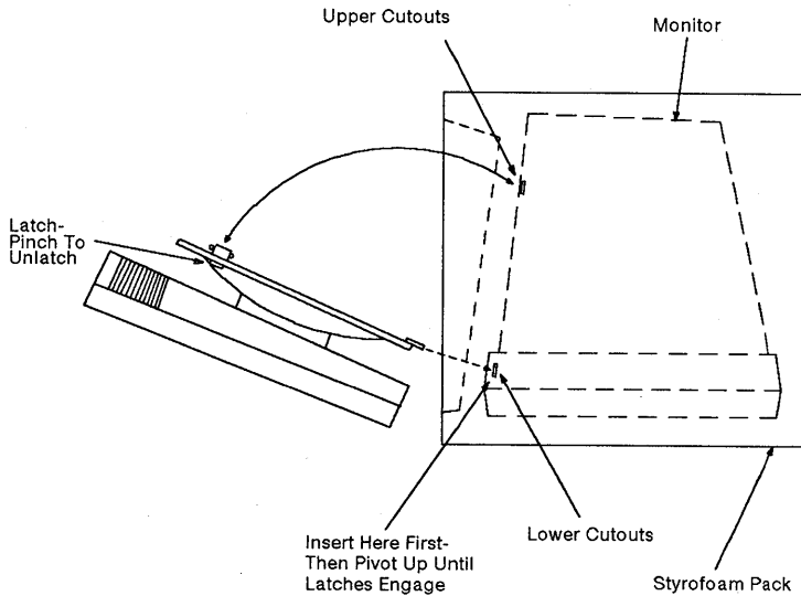
Figure 2-6 Attaching the Base to the Display
