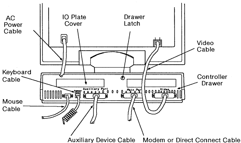
Figure 2-7 630 MTG (Rear View)
