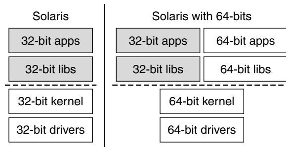
FIGURE 2-1 The Solaris Operating Environment Architecture
